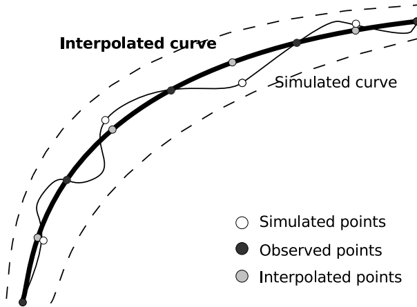
Fig. 1. The pollution trajectory curve.
