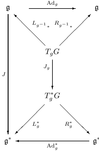
Fig. 2. Mappings between the spaces.
