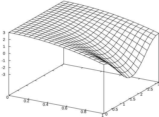
Fig. 1. The graph of 3 - 4s^2 + 2s^2 \cos 2\theta
