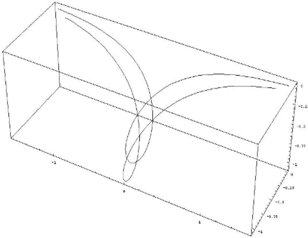
Fig. 1. Two curves (28) of one soliton solution of Manakov system, \epsilon_1 = \sqrt{2}/\sqrt{3} , \epsilon_2 = 1/\sqrt{3}
