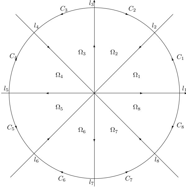
Fig. 1. The contours of integration \gamma_\nu = l_\nu \cup C_\nu \cup l_{\nu+1} .
