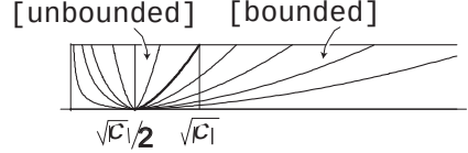
Fig. 4. Lamination on \mathcal{K}_2(\mathbb{C}H^n(c))
