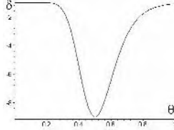
Fig. 1. The discriminant of the cubic characteristic equation in terms of \theta , for \gamma = 4 .
