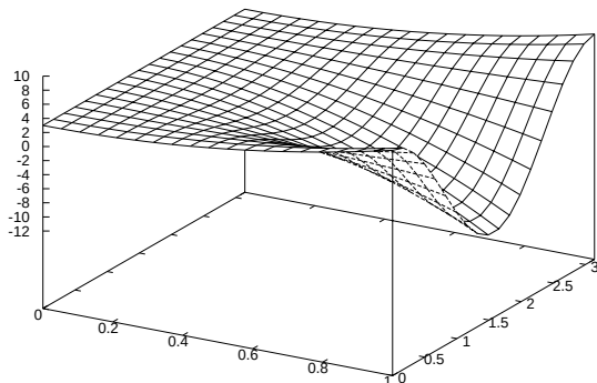
Fig. 2. The graph of 3 - 4s^2 + 10s^2 \cos 2\theta
