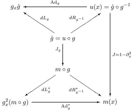
Fig. 3. Quantities related to the Camassa-Holm equation.
