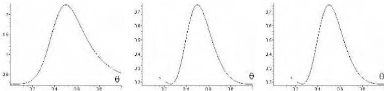
Fig. 3. The Jacobi eigenvalues in terms of \theta , for \gamma = 4 .
