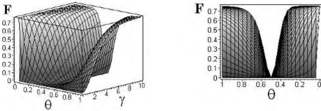
Fig. 5. The energy in terms of \theta and \gamma (general shape and projection onto \gamma = 0 ).
