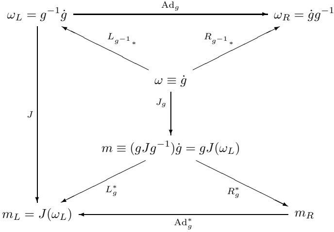
Fig. 1. Quantities and operators related to the \mathfrak{so}(3) algebra and its dual (Euler top case).
