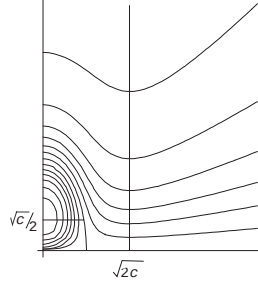
Fig. 6. Foliation on \mathcal{MK}_4(\mathbb{CP}^n)
