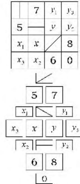
Figure 2: Conventions concerning a_{\alpha j}^k for p = 3 , \alpha = 1, 2, \dots, 5 ; a_{\alpha\lambda}^\lambda = 0 .
