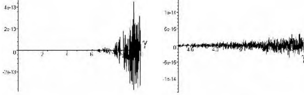
Fig. 4. The discriminant of the KCC characteristic polynomial in terms of \gamma , for \theta = 0.5 .
